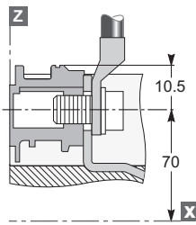
Cables with lugs/bars
