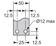
Top terminal
