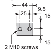
Top terminal
