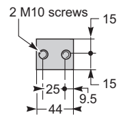
Bottom terminal
