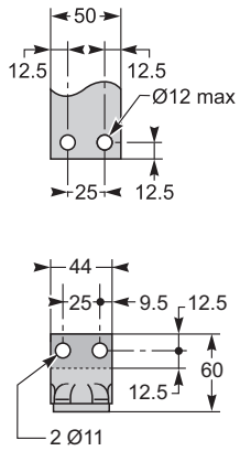
Rear connection
