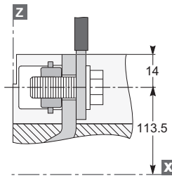
Bars/cables with lugs
