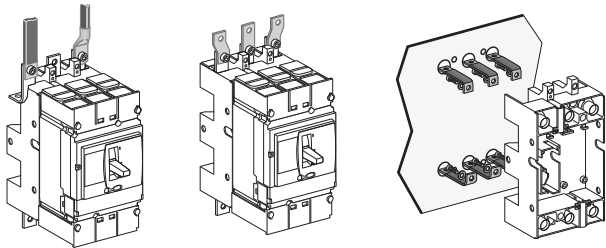
Front connection.
