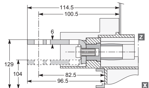
BX400/630
