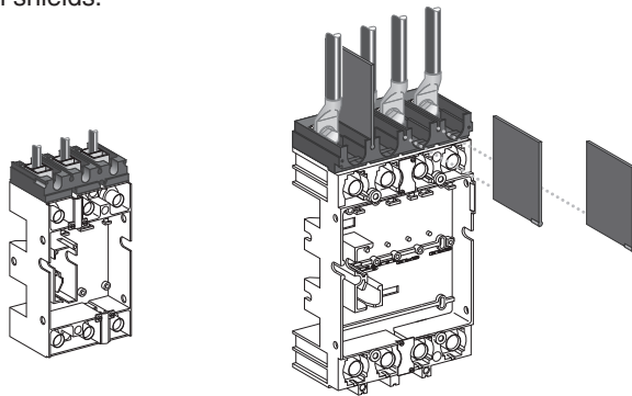
Adapter for 100 to 250 A - 3P base. Connection with bars or cables with lugs.
