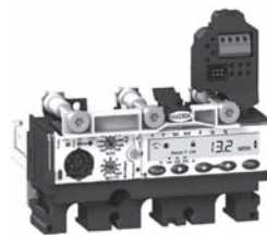
Control unit built-in LCD display showing an energy measurement.
