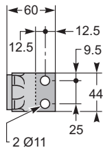
Vertical rear connection
