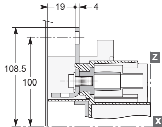
BX100 to 250
