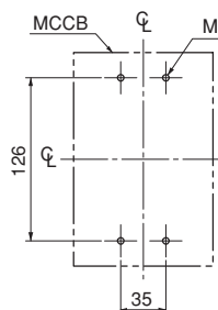
Panel drilling
