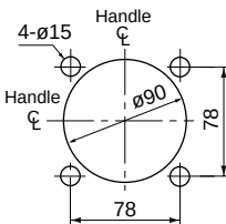
Door panel cutting
