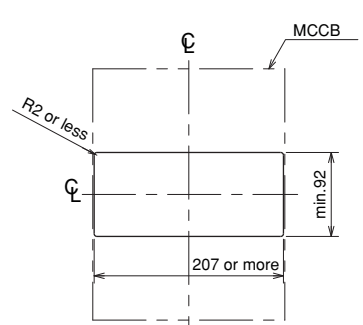
Front panel cutting
