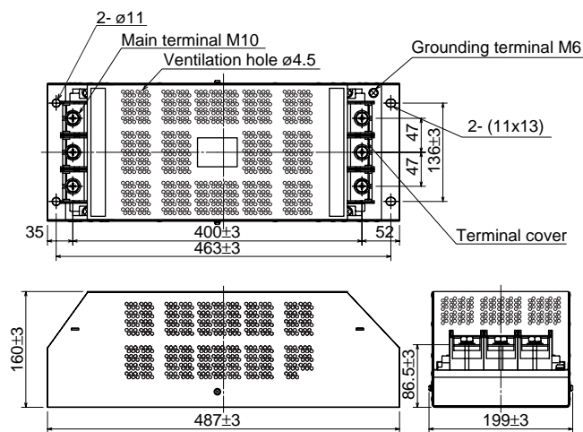
RNFMC3H-20, 40
