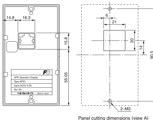
Panel cutting dimensions (view A)
