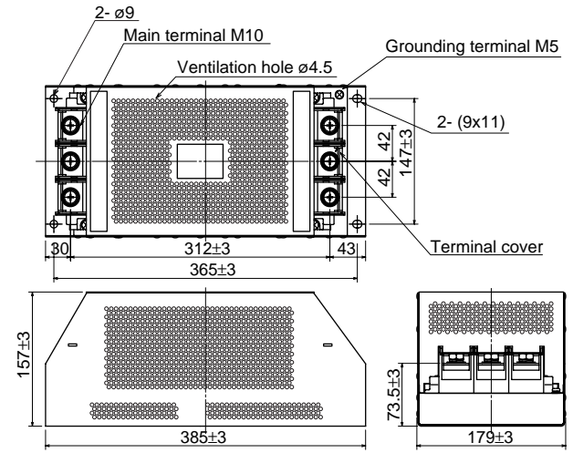
RNFMC2H-20, 40
