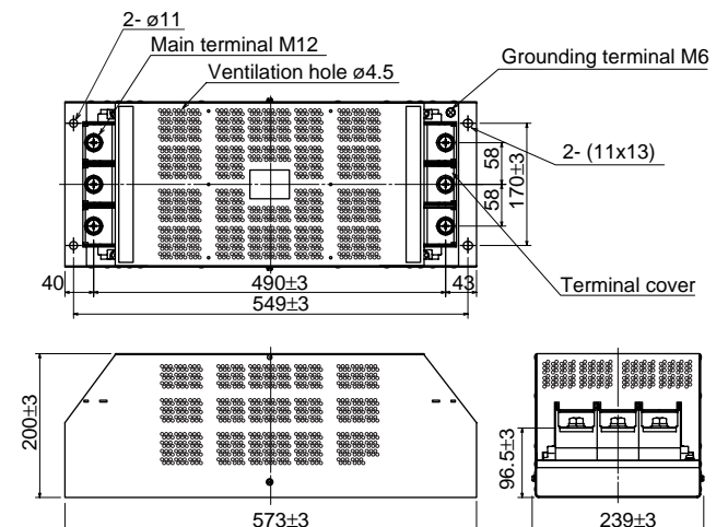
RNFMC4H-20, 40
